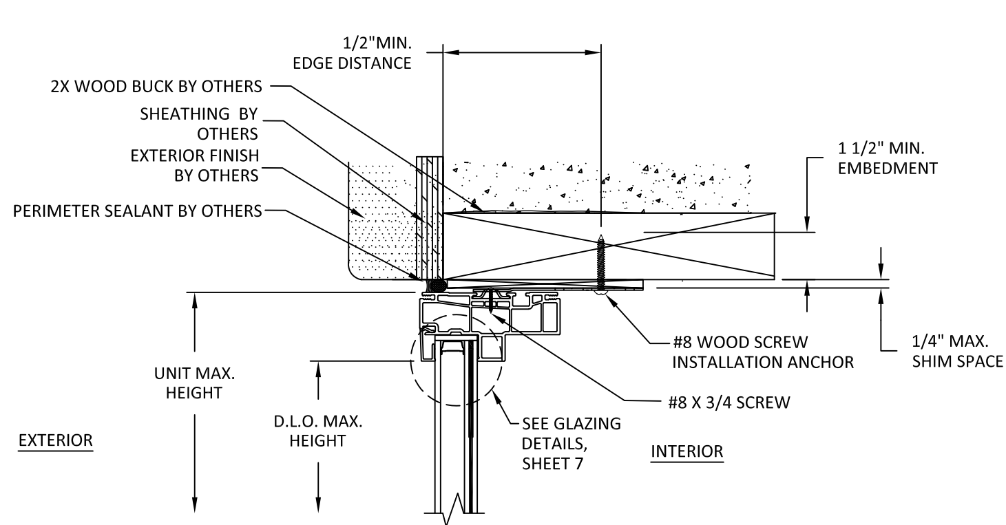
A 6 VERTICAL SECTION CLIP INSTALLATION WOOD SUBSTRATE
