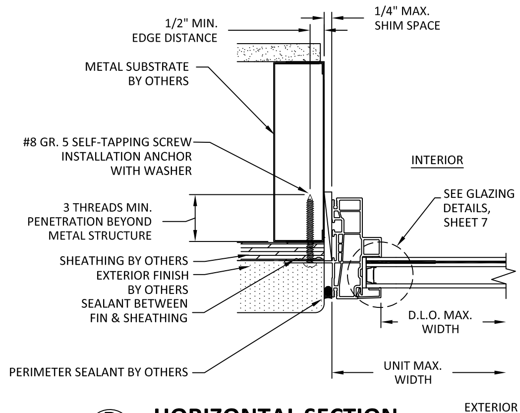
B 4 HORIZONTAL SECTION NAIL FIN INSTALLATION METAL SUBSTRATE
